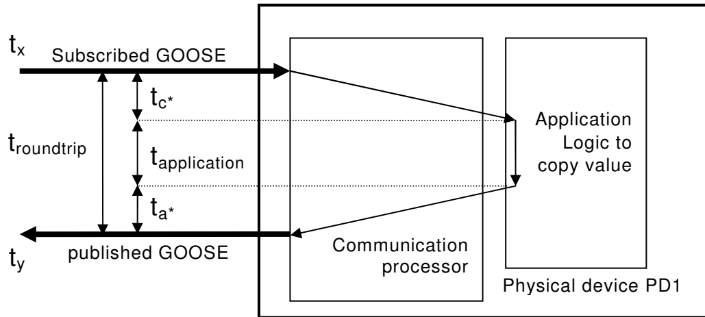
Figure 5 – Measure round trip time using GOOSE ping-pong method
