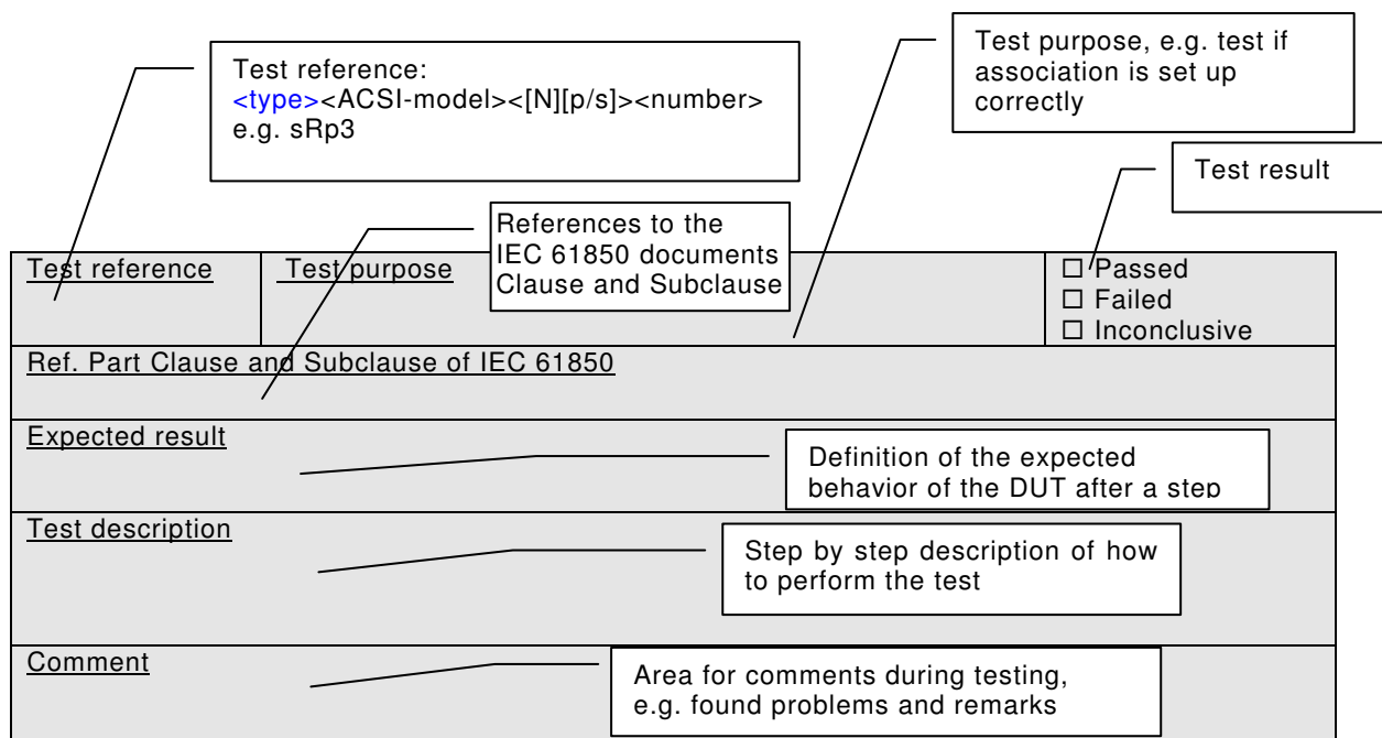
Figure 3 – Test procedure format
