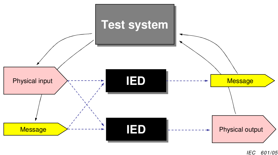
Figure 4 – Performance testing (black box principle)
