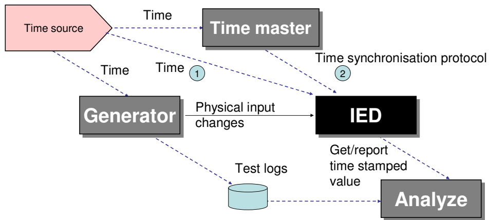
Figure 6 – Time synchronisation and accuracy test setup
