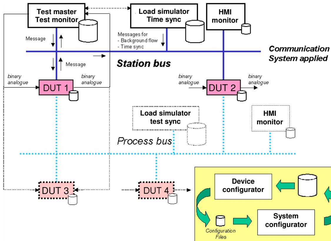
Figure 2 – Conceptual test system architecture
